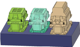
HDC, 1 2 3
